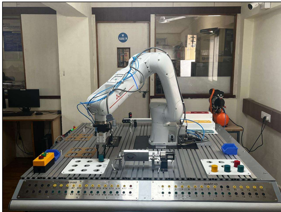
Figure 4: Manipulator performing workpiece placement in destination grid.
